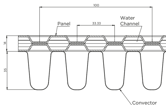
Radiator Section Detail
