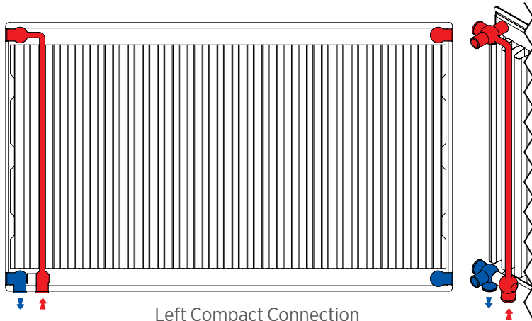
Left Compact Connection
