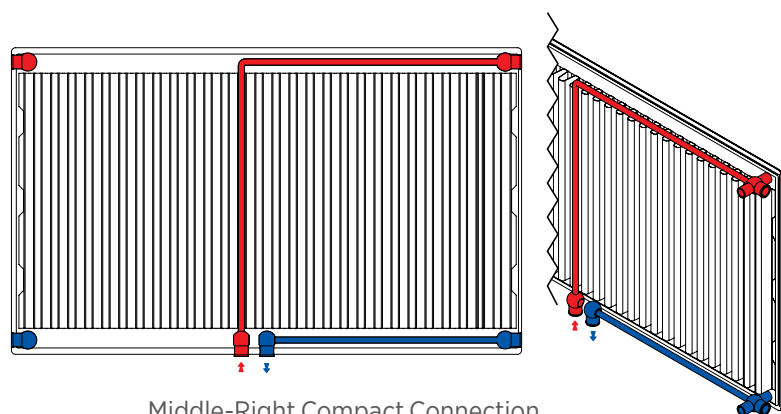
Middle-Right Compact Connection
