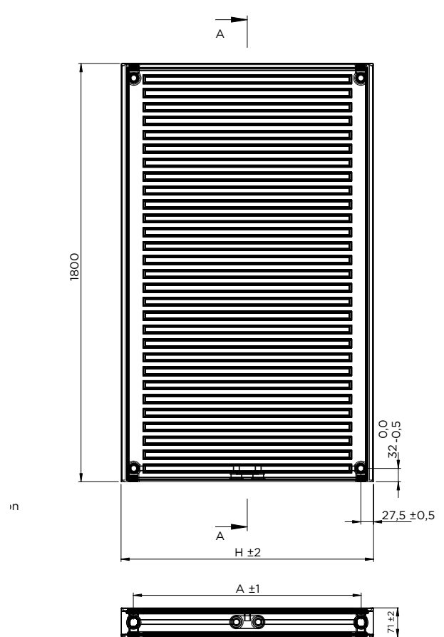
Type 20 Vertical Panel
